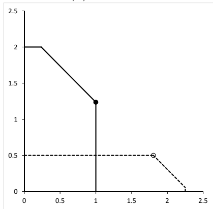
(c) \sigma_{G,1} = 2.25, \sigma_{G,2} = 0.5
