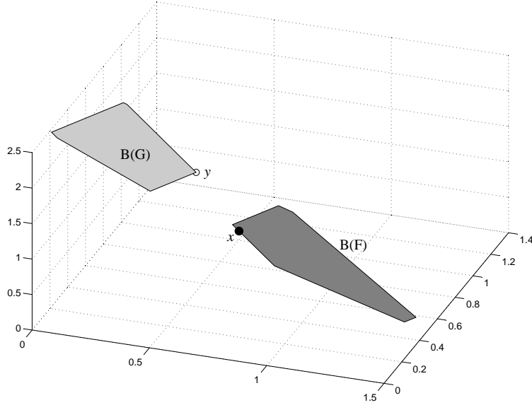
Figure 2: Base polyhedra and optimal attribution vectors for example (25)
